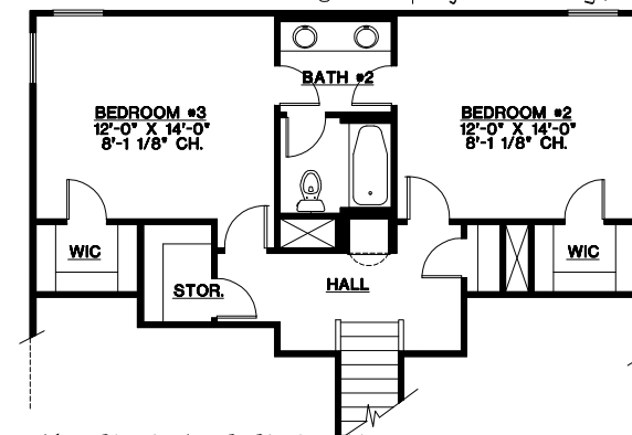
SECOND FLOOR PLAN 662 SQ.FT. EN-2670 Standard Floor Plan
